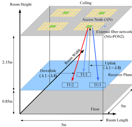
Fig. 1. LCoS-based access node in home area network
