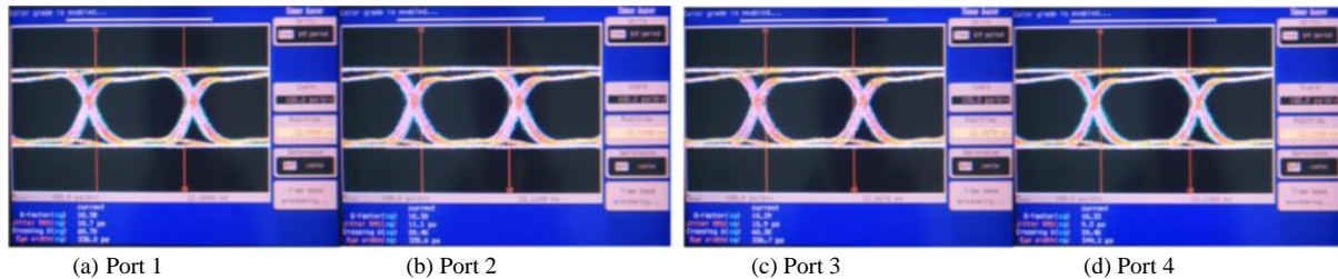
Fig. 4. Eye diagrams of a single wavelength transmitted from a TU is switched sequentially to four output ports of the node. ( \lambda = 1555.6 \text{ nm} )
