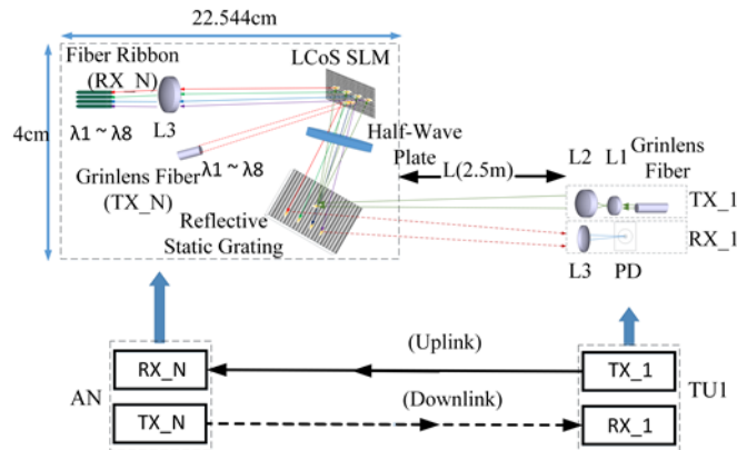
Fig. 2. Ray tracing of proposed node architecture in up/down link
