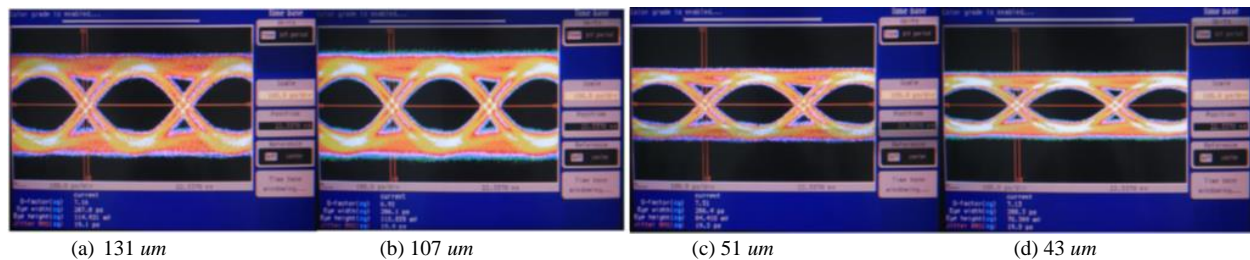
Fig. 5. Eye diagrams taken when the spot size focused at TU in downlink was expanded from 43 \mu\text{m} to 131 \mu\text{m} ( \lambda = 1550 \text{ nm} )
